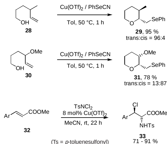
Scheme 7 Copper(II) triflate promoted electrophilic additions to olefins
