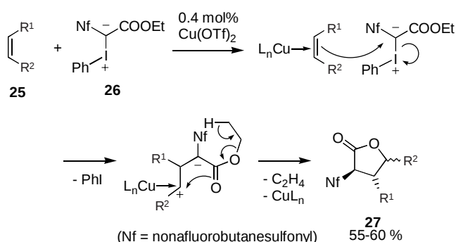
Scheme 6 Olefin activation by means of copper(II) triflate; synthesis of \gamma -lactones
