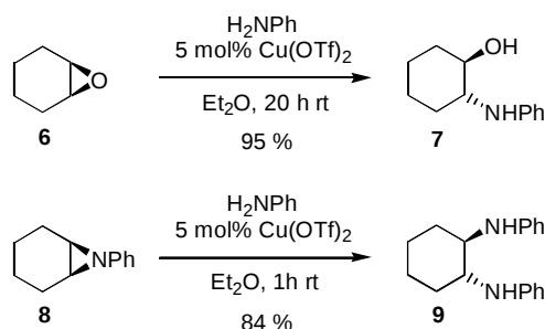
Scheme 3 Ring-opening of epoxides and aziridines
