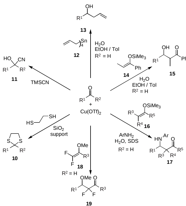
Scheme 4 Copper(II) triflate catalyzed reactions of carbonyl compounds
